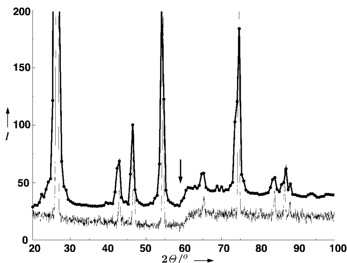
Figure 5. Selected area of the neutron diffraction pattern (lower curve) with the step-like diffuse scattering and simulated pattern (upper curve).
